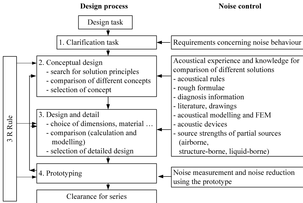
Fig. 1. Stages of acoustic ecodesigning.
